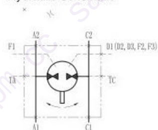
Hydraulic Schematic
