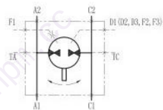
Hydraulic Schematic
