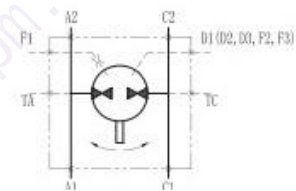
Hydraulic Schematic
