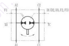
Hydraulic Schematic
