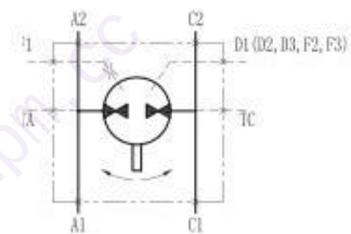
Hydraulic Schematic
