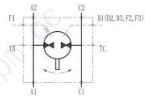
Hydraulic Schematic
